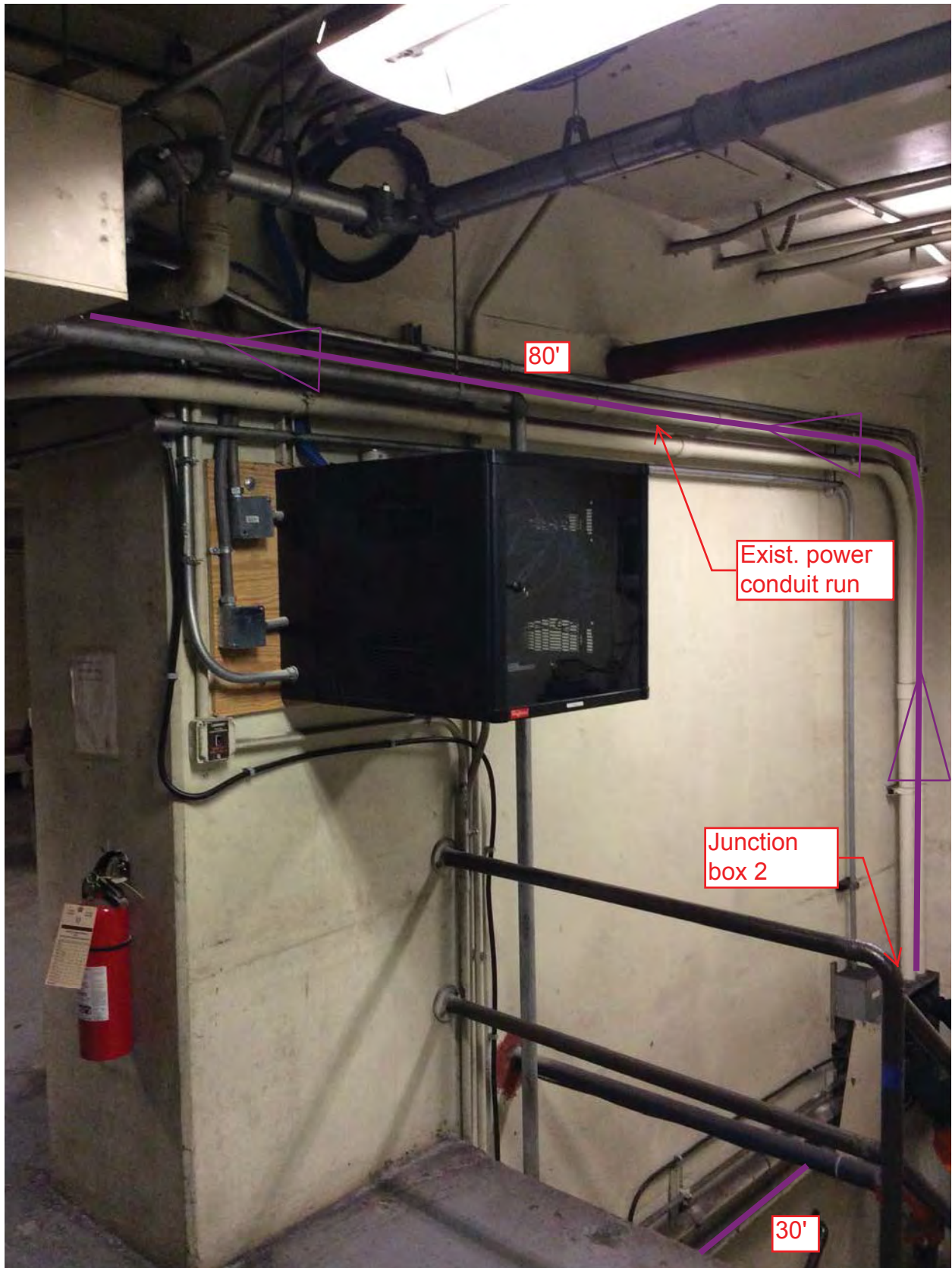
Picture 9: D07 Potomac Ave – Existing conduit from junction box 2 toward AFC Panel
