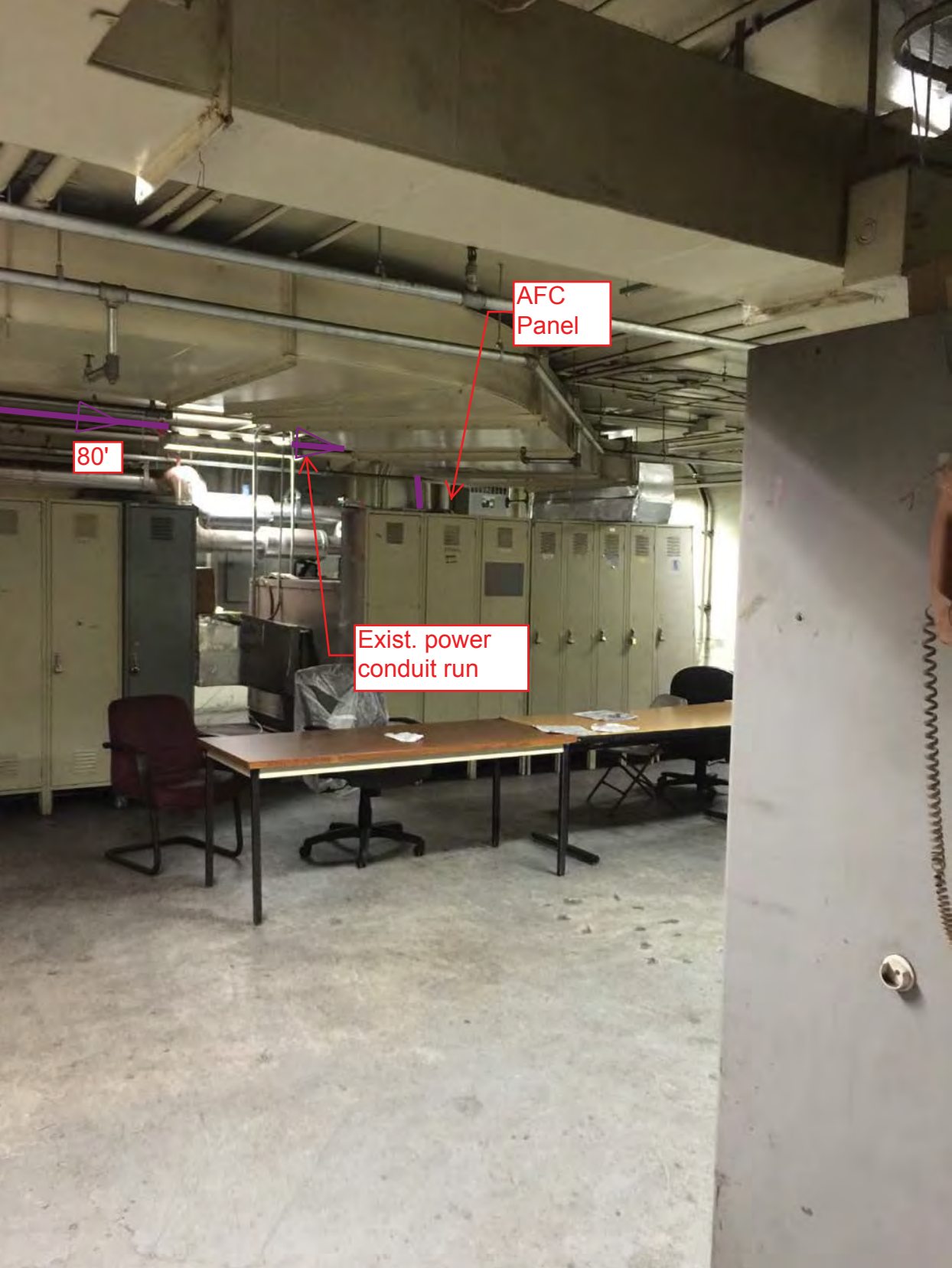
Picture 12: D07 Potomac Ave – Existing conduit from junction box 2 toward AFC Panel
